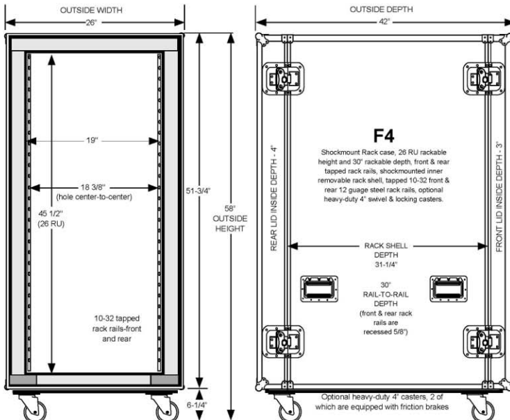
Rack Shown -Stock Model Quick Ship OEMRACF4X26X30
