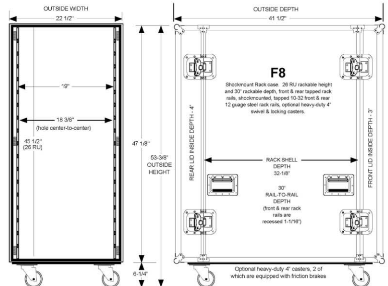
Rack Shown - Custom Model F8X26X30
